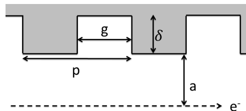
Figure 2: Dimensions of corrugated plates. See Table 1.
