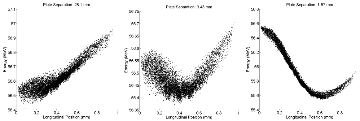
Figure 3: Longitudinal phase space plots at various plate gaps as simulated in Elegant. Note that the smallest gap causes an overchirp that results in a larger energy spread.
