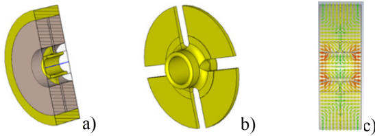
Figure 3: \pi -mode, \beta_{ph}=0.34 DaR cell cut view with Alumina rings (a), copper disk (b), and electric fields (c).
