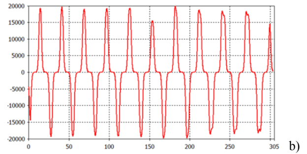
Figure 7: Longitudinal electric field profiles simulated along DaR MicroLinac for operating modes at \sim 9.4 GHz for the 1 st (a) and 2 nd (b) sections of Fig. 5.
