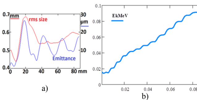
Figure 13: Beam rms sizes and normalized emittance (a) as well as energy gain (b) along the short focusing section of Fig. 12 and initial part of structure shown in Fig. 5a.
